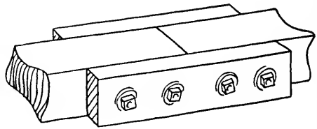
FISHED JOINT-B
